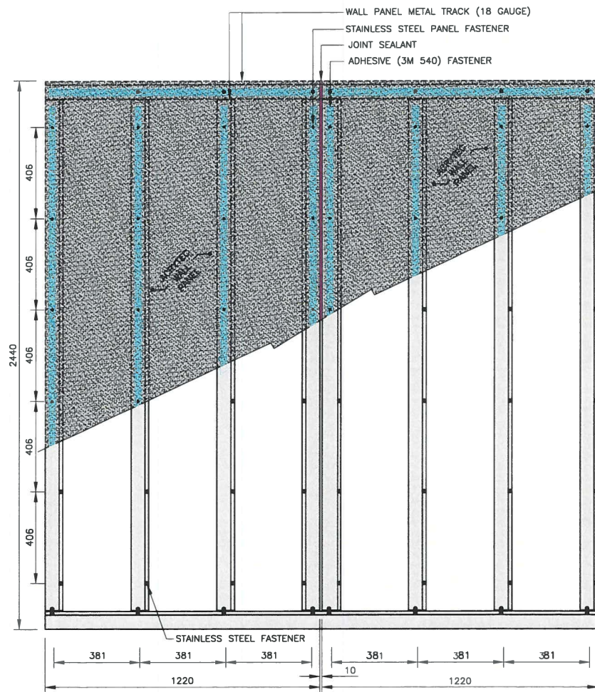
○ PARTIAL ELEVATION Scale: 1:10
